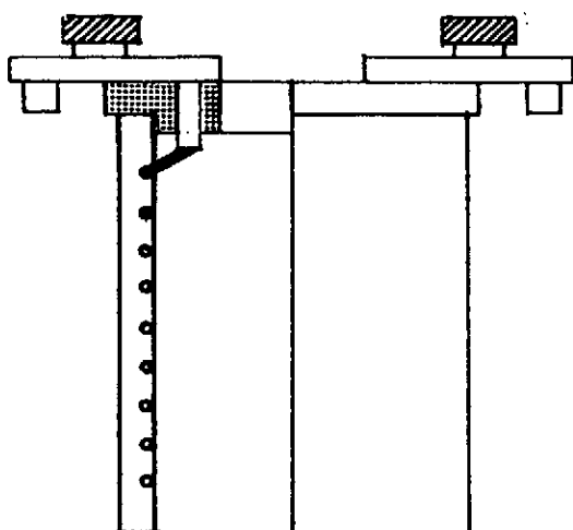
FIGURE 3 A Thomas 1 \Omega Resistor (After Leeds and Northrup)
